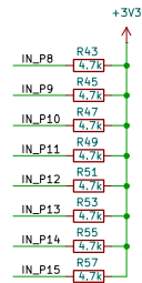
Input Terminal Block 2
